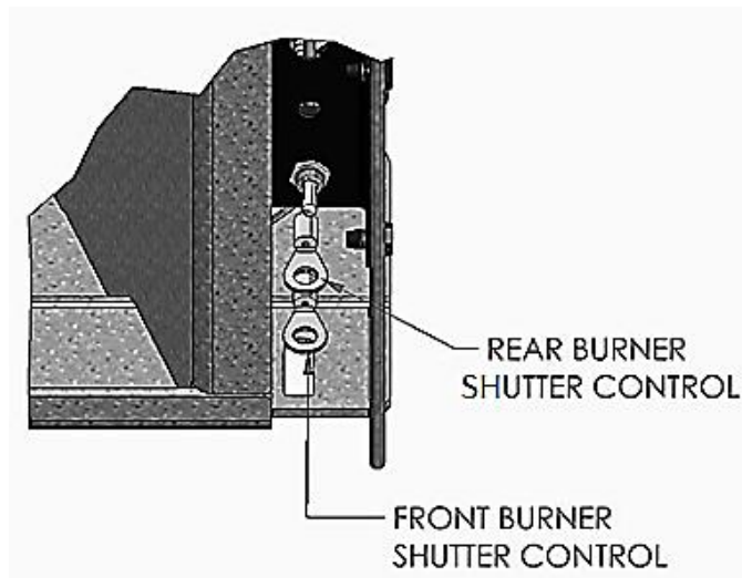
Burner Air Shutter Controls
