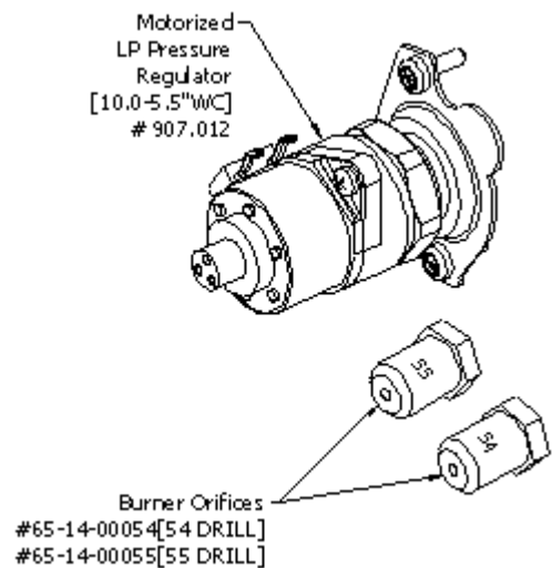
HA-58-00302 LP Kit Parts
