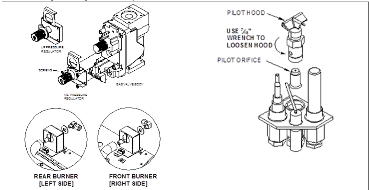
Figure 4-3 Conversion Preparation
