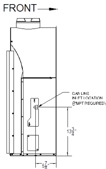
Figure 3-18 Gas Line Inlet Location
