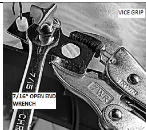
Figure 4-7 Pinch Pilot Base with Vice Grips
