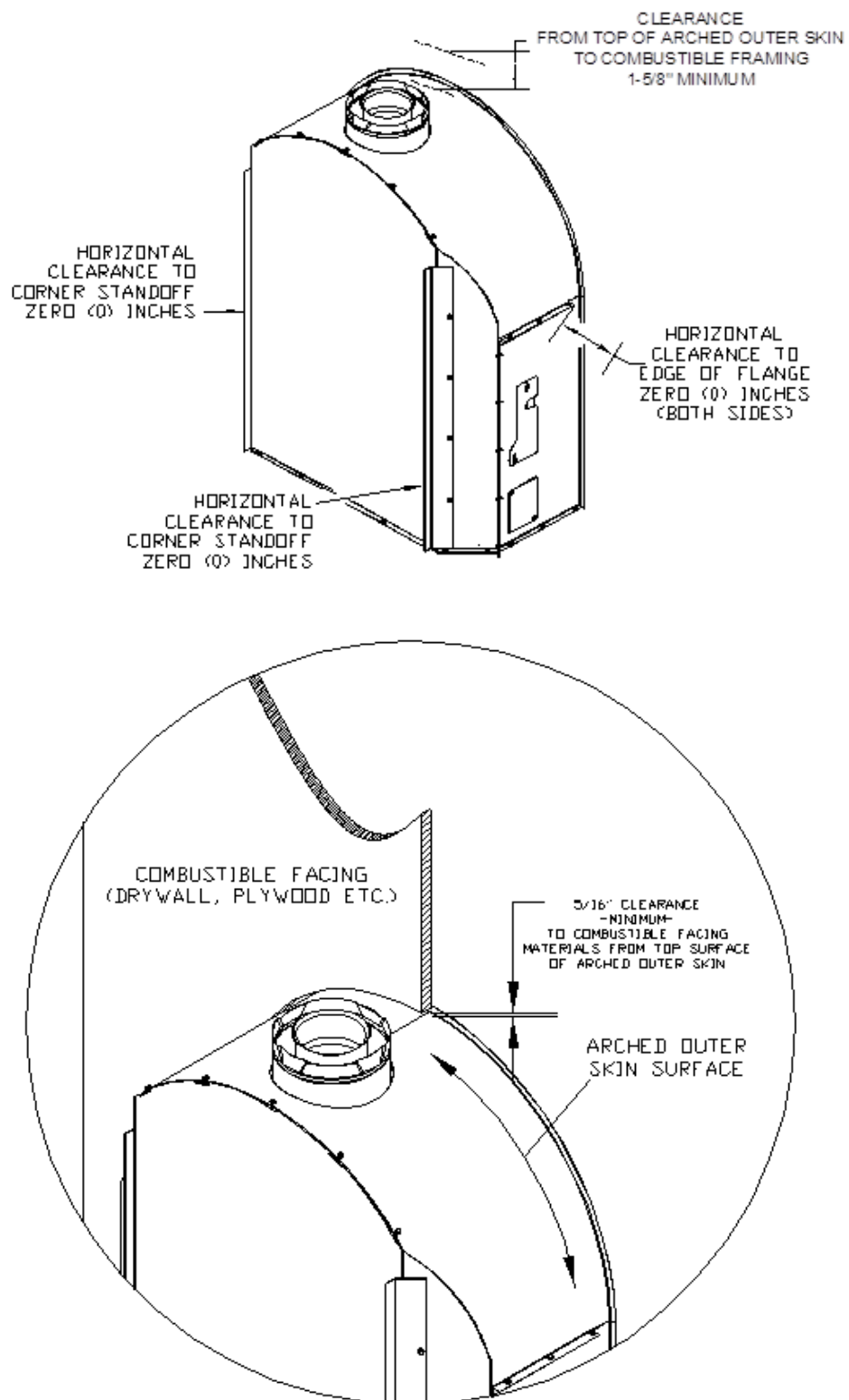
Figure 3-7 CLEARANCES TO APPLIANCE BODY
