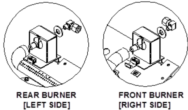
Figure 4-5 Removing Orifices
