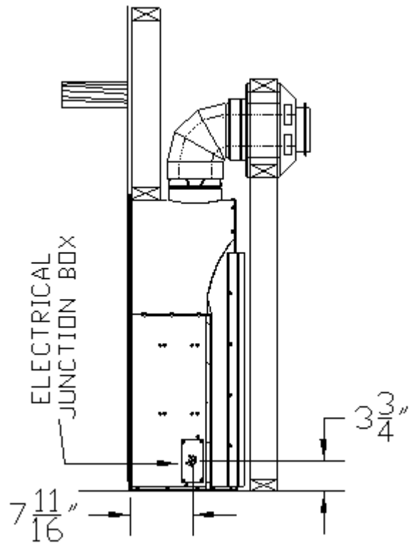
Figure 3-15 Electrical Junction Box
