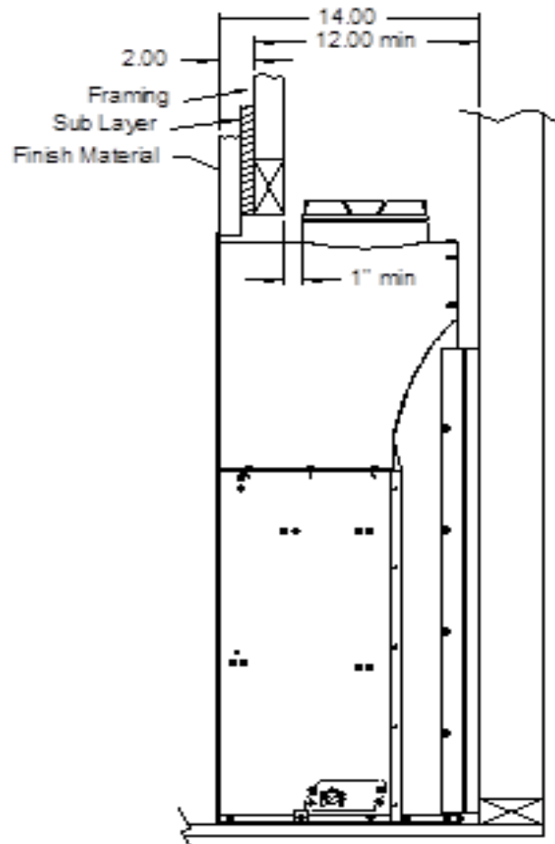
Figure 3-13 FRAMING DEPTH/ FINISHING MATERIAL THICKNESS
