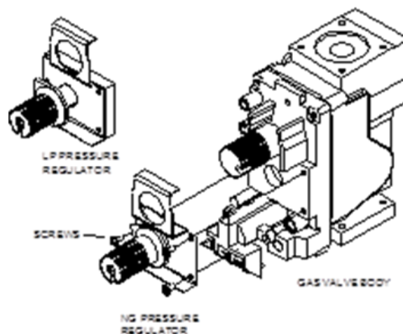
Figure 4-4 Pressure Regulator Conversion
