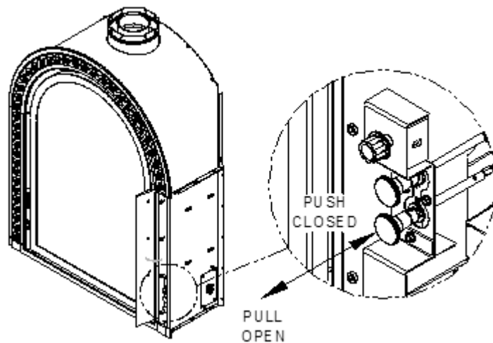
Figure 4-8 Burner Air Shutter Controls
