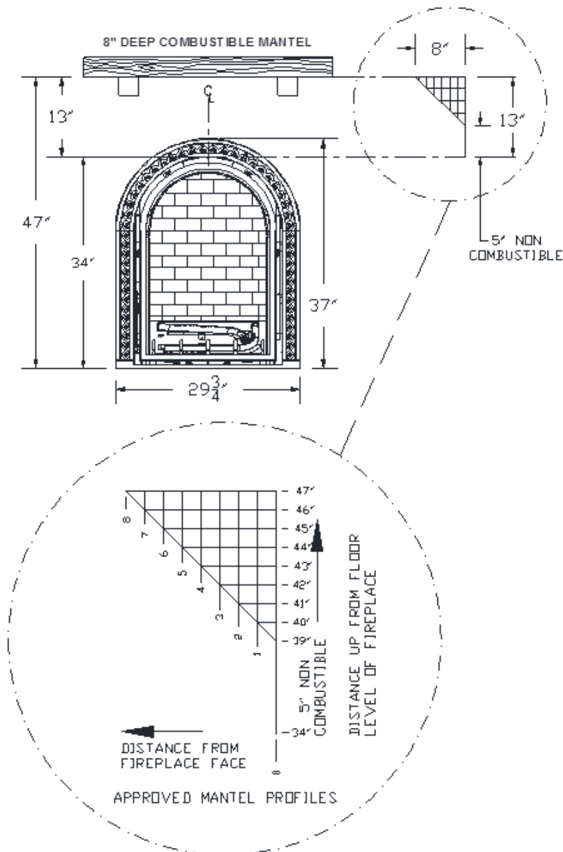
Figure 3-9 Mantel Clearances
