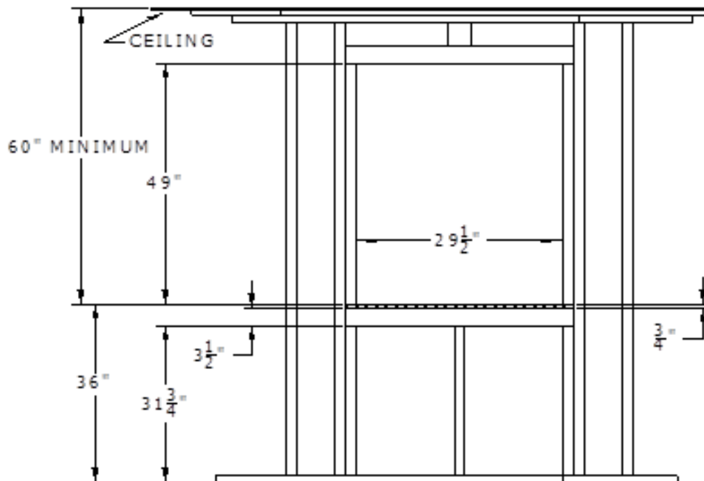
Figure 3-6 ELEVATED FRAMING DIMENSIONS
