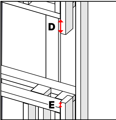
Alternate view for open-sided installation.
